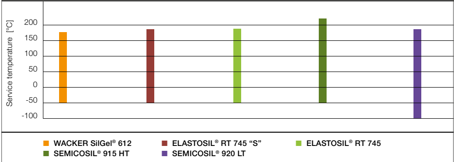
Chart 4: WACKER Silicone Gels, Service Temperature
