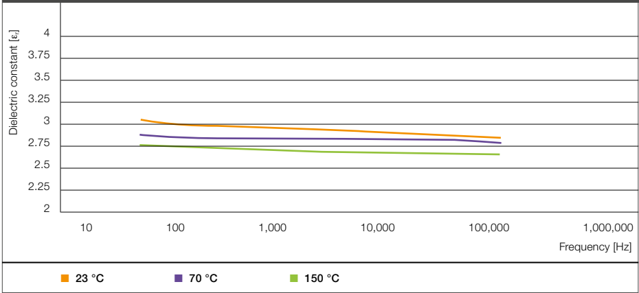
Chart 3: WACKER SilGel® 612, Dielectric Constant
